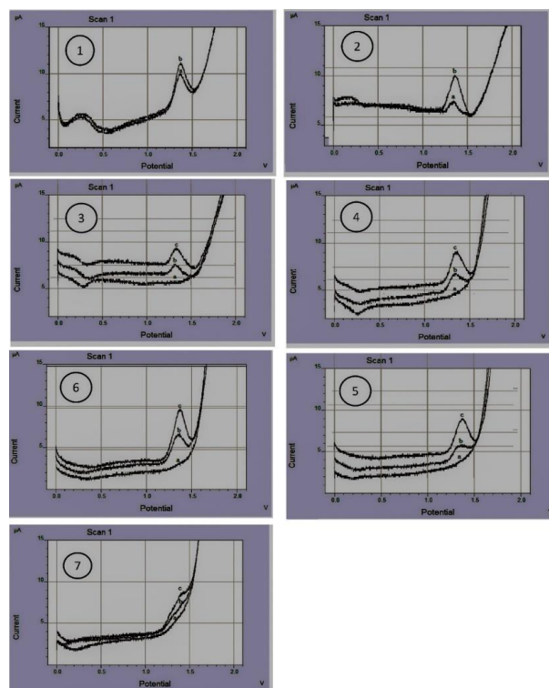
Figure 1. Voltammograms obtained for 50 and 100 mg/L 2,4-D standard solutions in different pH environments. 1: a) 50 mg/L 2,4-D in pH 2 BRT buffer b) 100 mg/L 2,4-D; 2: a) 50 mg/L 2,4-D b) 100 mg/L 2,4-D in pH 3 BRT buffer; 3: in pH 4 BRT buffer a) 10 mL pH 4 BRT buffer b) 50 mg/L 2,4-D c) 100 mg/L 2,4-D; 4: in pH 5 BRT buffer a) 10 mL pH 4 BRT buffer b) 50 mg/L 2,4-D c) 100 mg/L 2,4-D; 5: in pH 6 BRT buffer a) 10 mL pH 4 BRT buffer b) 50 mg/L 2,4-D c) 100 mg/L 2,4-D; 6: in pH 7 BRT buffer a) 10 mL pH 4 BRT buffer b) 50 mg/L 2,4-D c) 100 mg/L 2,4-D; 7: in pH 8 BRT buffer a) 10 mL pH 4 BRT buffer b) 50 mg/L 2,4-D c) 100 mg/L 2,4-D.
