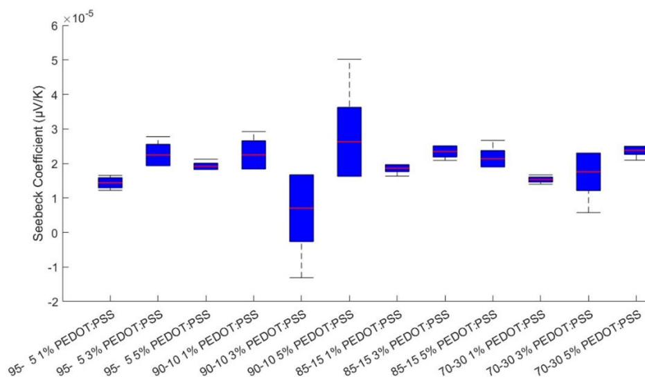
Figure 6. The Seebeck Coefficient measurements of films prepared with different ratios of PEDOT: PSS was added to DMSO-water solutions of varying concentrations.
