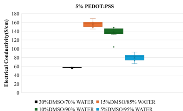
Figure 1. The electrical conductivities of films prepared with 5% PEDOT: PSS added to DMSO-water mixtures at different concentrations.
