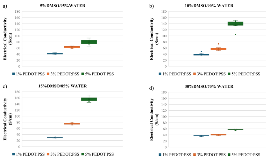
Figure 5. The electrical conductivities of films prepared with different ratios of PEDOT: PSS was added to DMSO-water solutions of varying concentrations a) 5% DMSO/95% water b) 10% DMSO/90% water c) 15% DMSO/85% water d) 30% DMSO/70% water.
